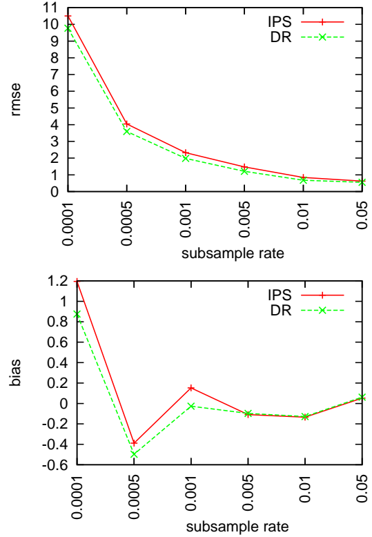
Figure 3. Comparison of IPS and DR: rmse (top), bias (bottom). The ground truth value is 23.8.
