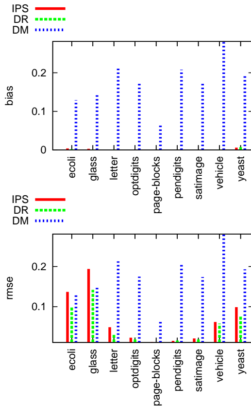
Figure 1. Bias (upper) and rmse (lower) of the three estimators for classification error. See Table 2 for precise numbers.
