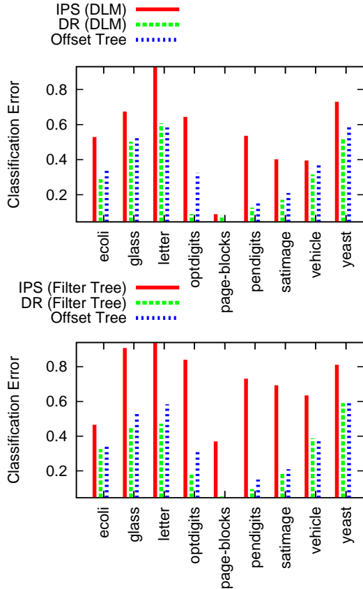
Figure 2. Classification error of DLM (upper) and filter tree (lower). Note that the representations used by DLM and the trees differ radically, conflating any comparison between the approaches. However, the Offset and Filter Tree approaches share a similar representation, so differences in performance are purely a matter of superior optimization. See Table 3 for precise numbers.
